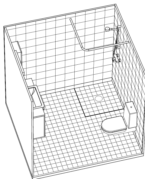
Fig. 1 Bathsystem prefabricated bathroom modules, principle construction
